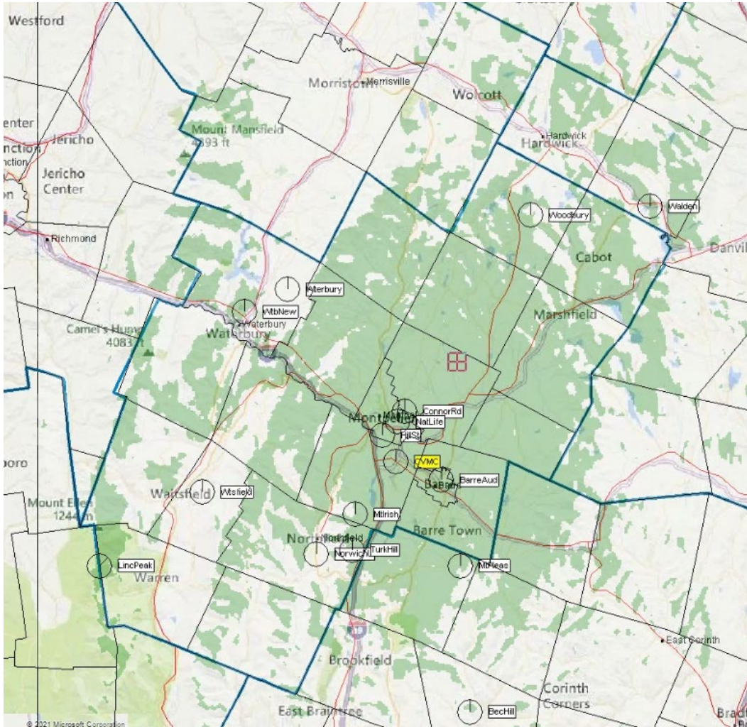
Figure 15: Current Predicted Coverage for Ambulance to Hospital Communications
